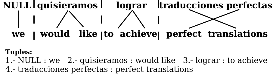
Figure 1: Example of tuple extraction.
