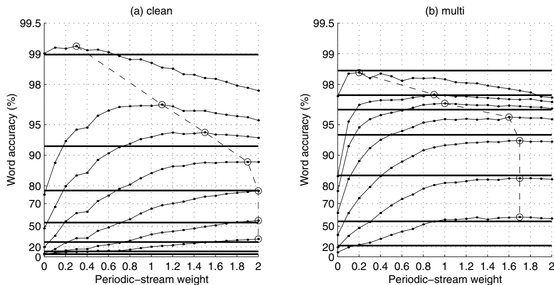
Figure 4: SPLIT test results of word accuracy (%) versus periodic-stream weight \gamma_p , averaged across each noise level: (a) clean and (b) multi-condition training. Solid lines are (from top): \infty , 20 dB, 15 dB, 10 dB, 5 dB, 0 dB and -5 dB SNR test conditions. Thick horizontal lines indicate baseline average scores, and the dashed line (with \odot ) indicates the best at each noise level.
